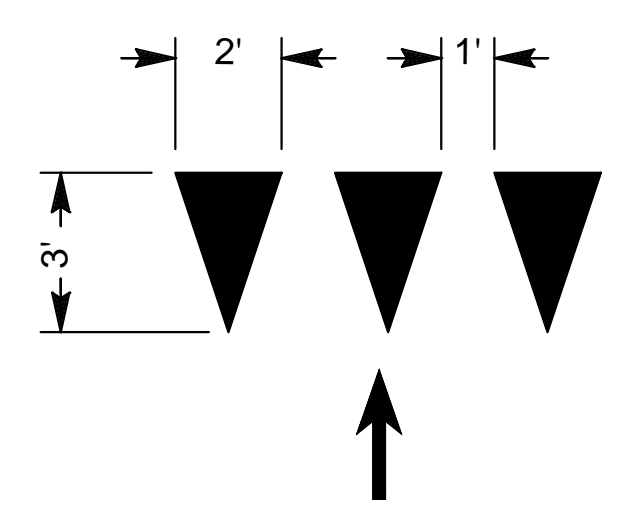
DIRECTION OF TRAVEL DETAIL E YIELD LINE N.T.S.
